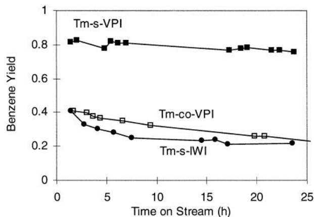
FIG. 2. Yield of benzene as a function of time on stream (WHSV, 5 h -1 ) for Tm-s-VPI, Tm-co-VPI, and Tm-s-IWI catalysts.
